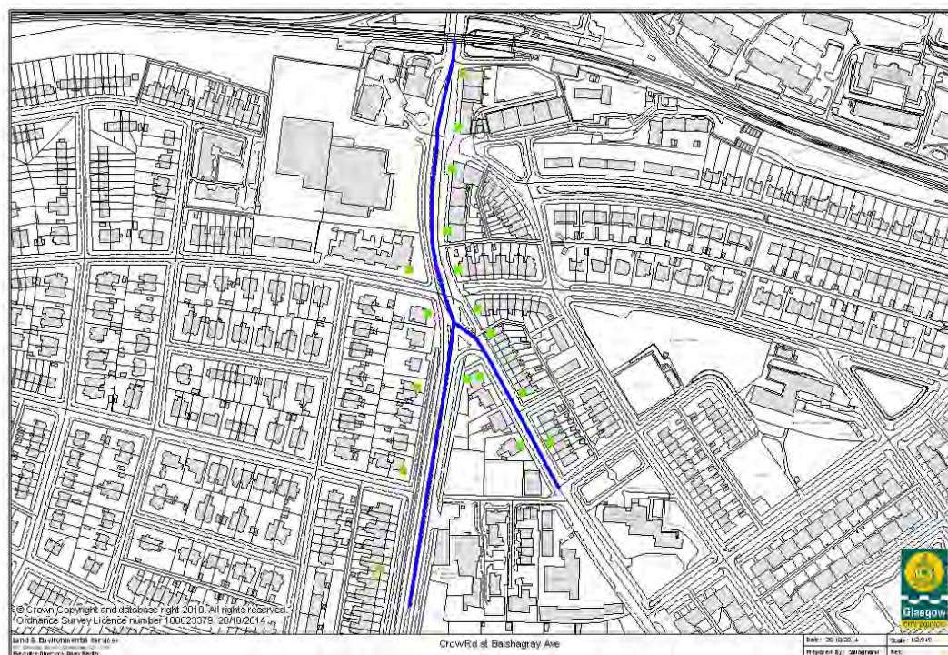
Figure 3.17 Crow Rd at Balshagray Ave modelled streets and receptors
