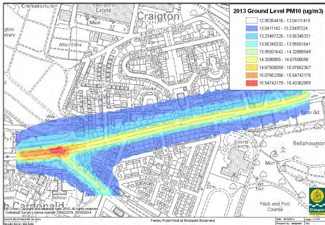
Figure 3.48 Paisley Road West at Mosspark Boulevard PM 10 contours
