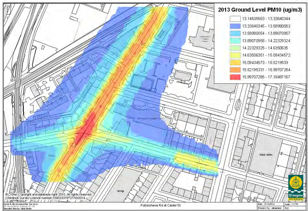
Figure 3.40 Pollokshaws Rd at Calder St Rd PM 10 contours
