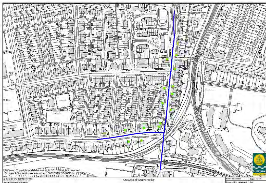
Figure 3.19 Crow Rd at Southbrae Dr modelled streets and receptors
