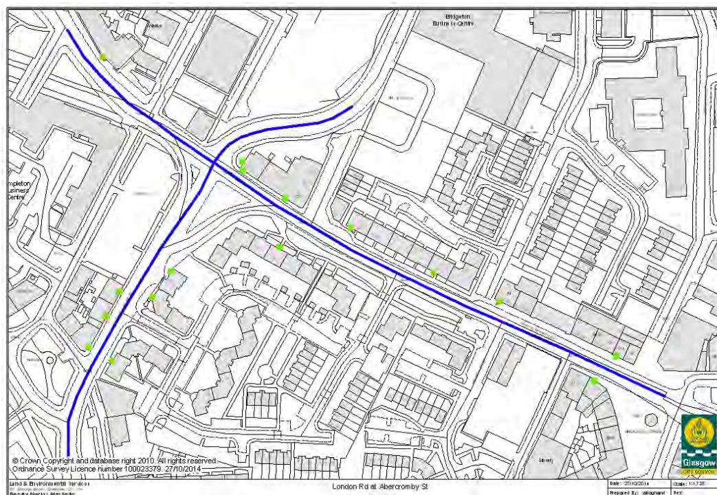
Figure 3.31 London Rd at Abercromby St modelled streets and receptors
