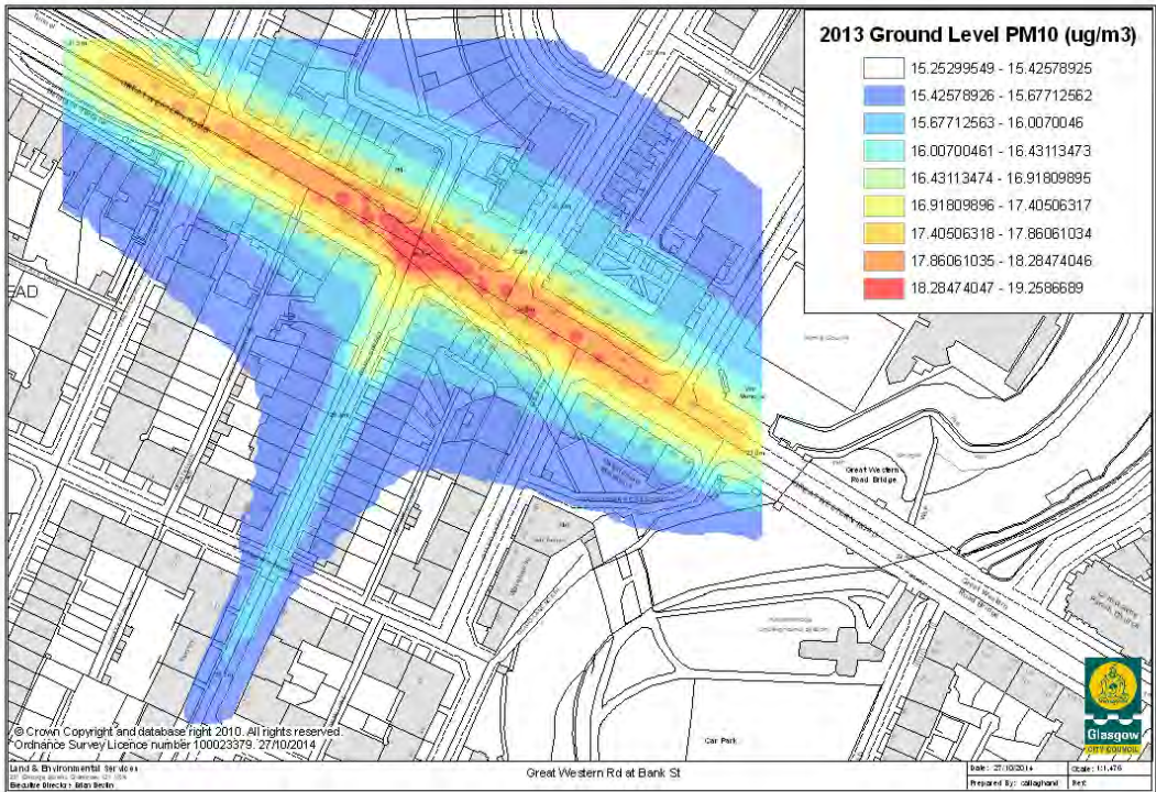
Figure 3.26 Great Western Rd at Bank St PM 10 contours
