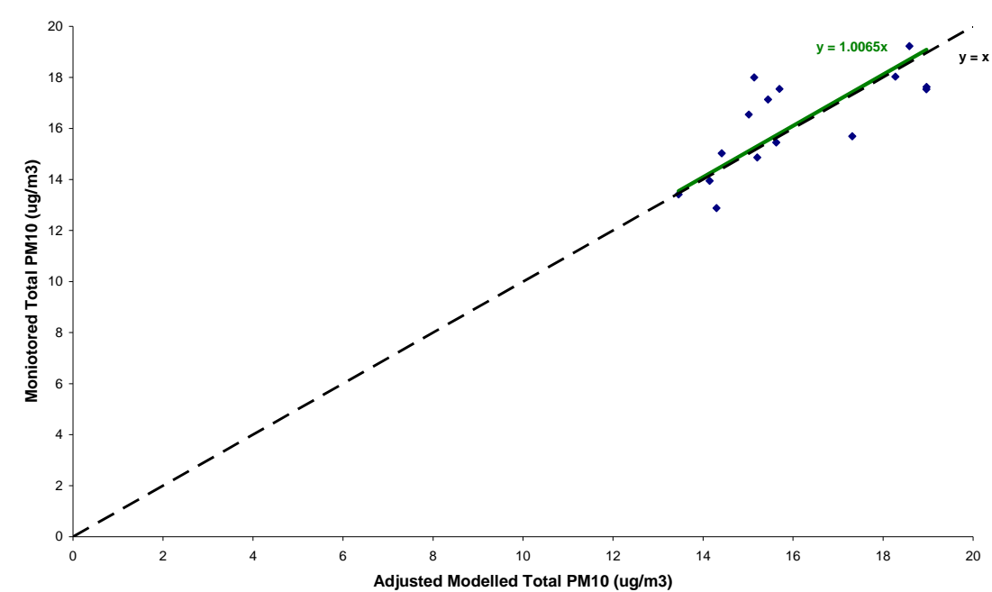
Figure 2.8 adjusted modelled vs monitored annual average PM 10
