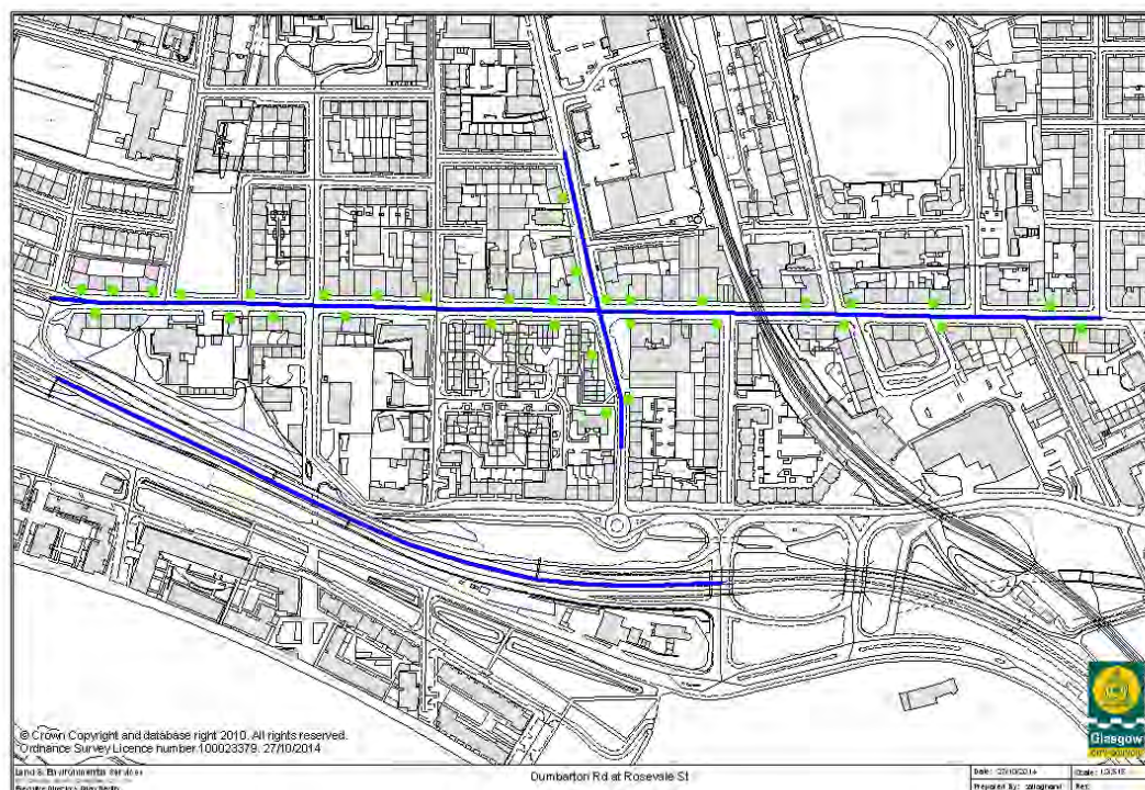
Figure 3.23 Dumbarton Rd at Rosevale St modelled streets and receptors
