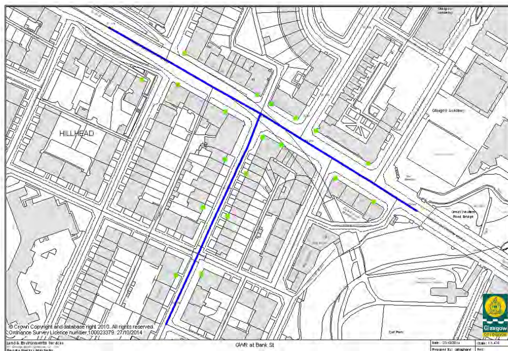
Figure 3.25 Great Western Rd at Bank St modelled streets and receptors
