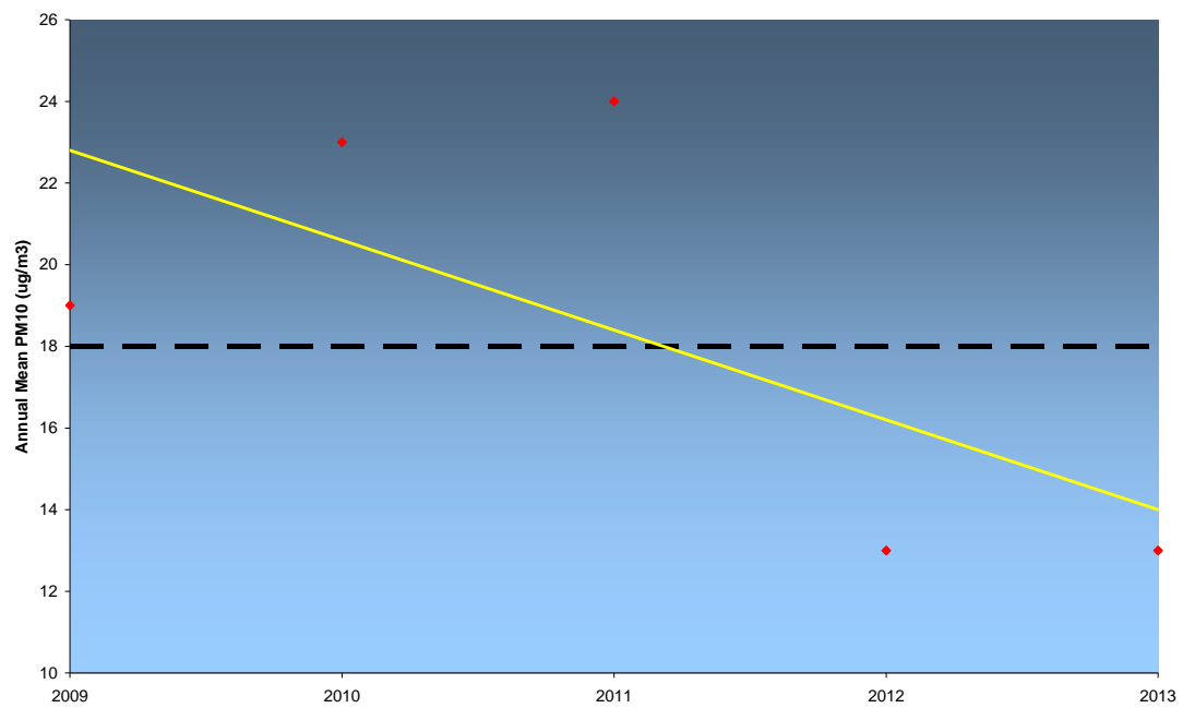
Figure 3.4 Glasgow Byres Rd PM 10 trend
