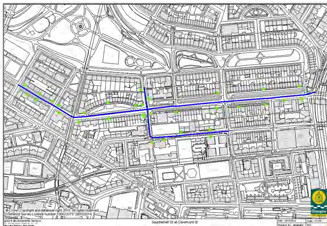
Figure 3.49 Sauchiehall St at Claremont St modelled streets and receptors
