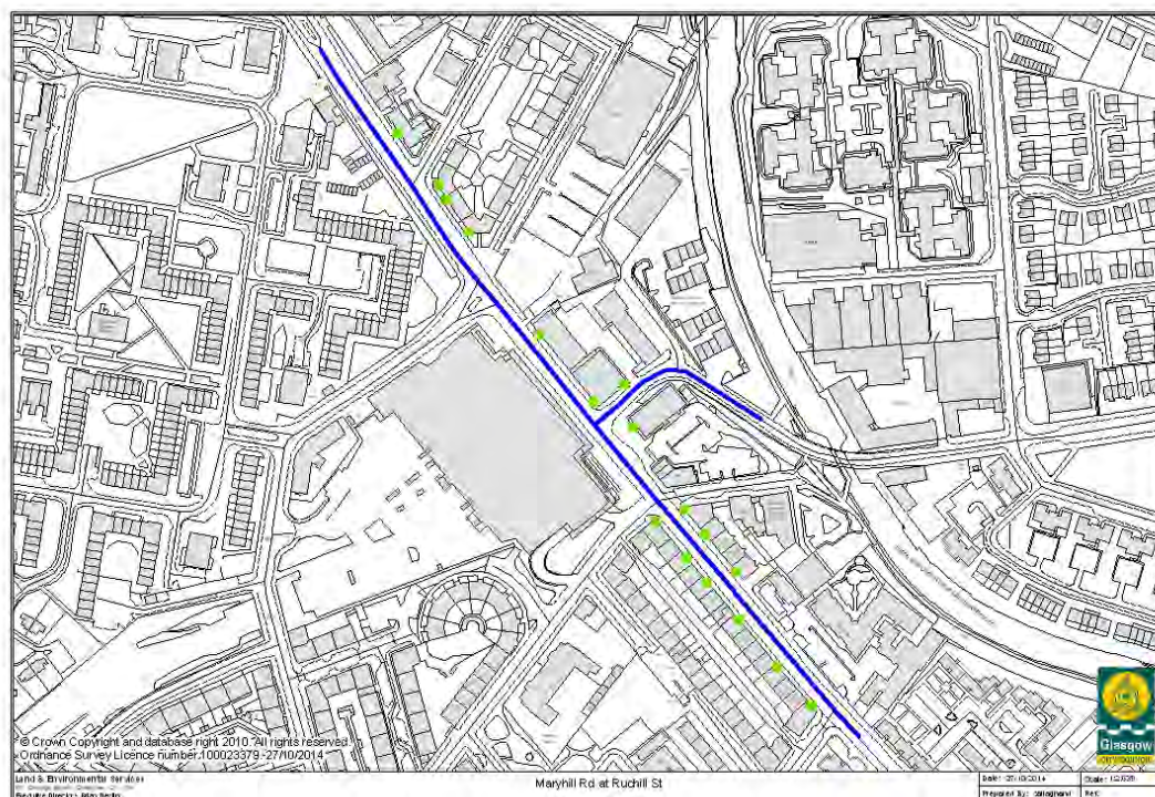
Figure 3.35 Maryhill Rd at Ruchill St modelled streets and receptors
